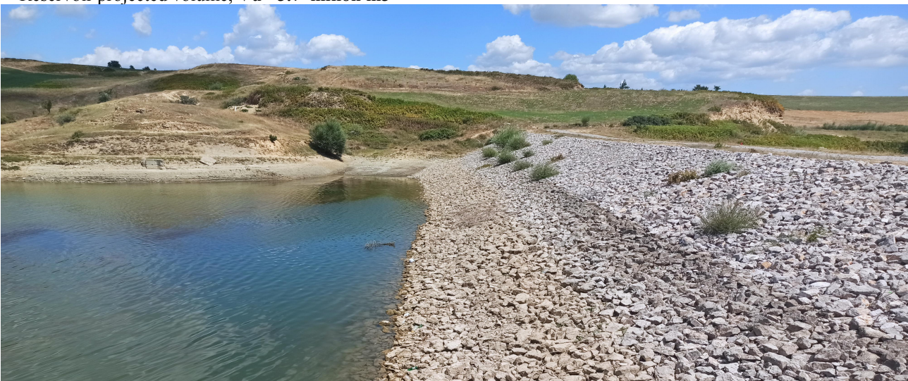
6- Irrigation dam and reservoir of Koshnica, Devoll, H = 31.0 m, Reservoir projected volume, Vu= 3.7 milion m3
